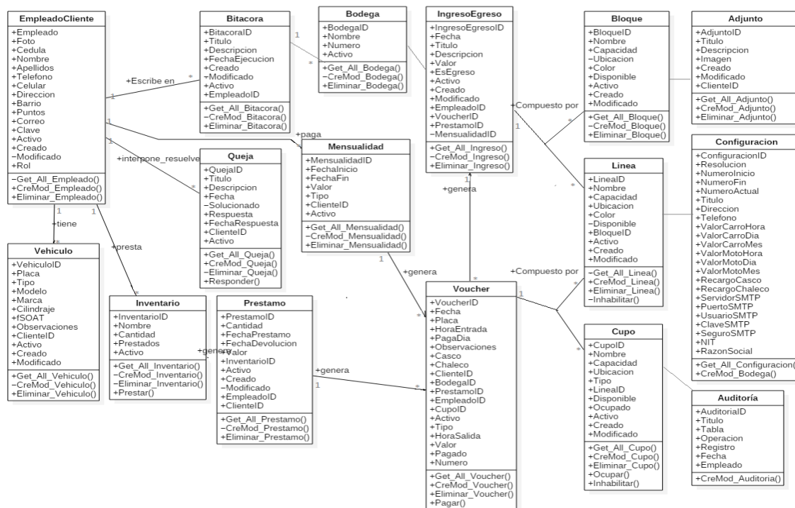
Figure 2. Class diagram
