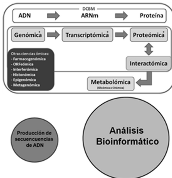
Figure 1. Development of omics sciences through the flow of genetic information or CDMB (*), above. Changes in infrastructure requirements of the genome project, below.
