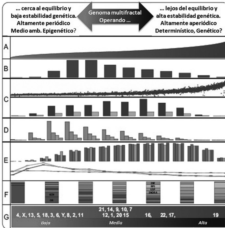
Figure 6. MFA summary diagram of the HG. From left to right the multifractality increases. Adapted from Moreno et al , 2011.
