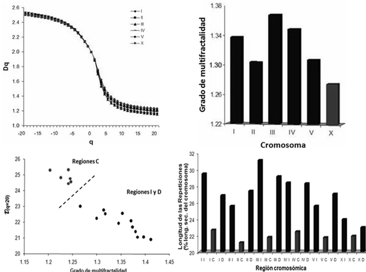
Figure 5. MFA for the C. elegans genome. Multifractal spectra and distribution of multifractality by chromosome, above. 2-D discrimination analysis by chromosome region and distribution of repeat length by chromosomal region, below.
