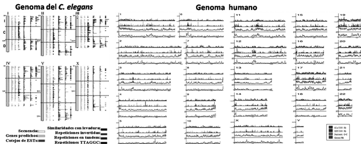
Figure 2. Map of the C. elegans genome by chromosome divided into three regions (L: left, C: central and R: right) and map of the HG by chromosome.
