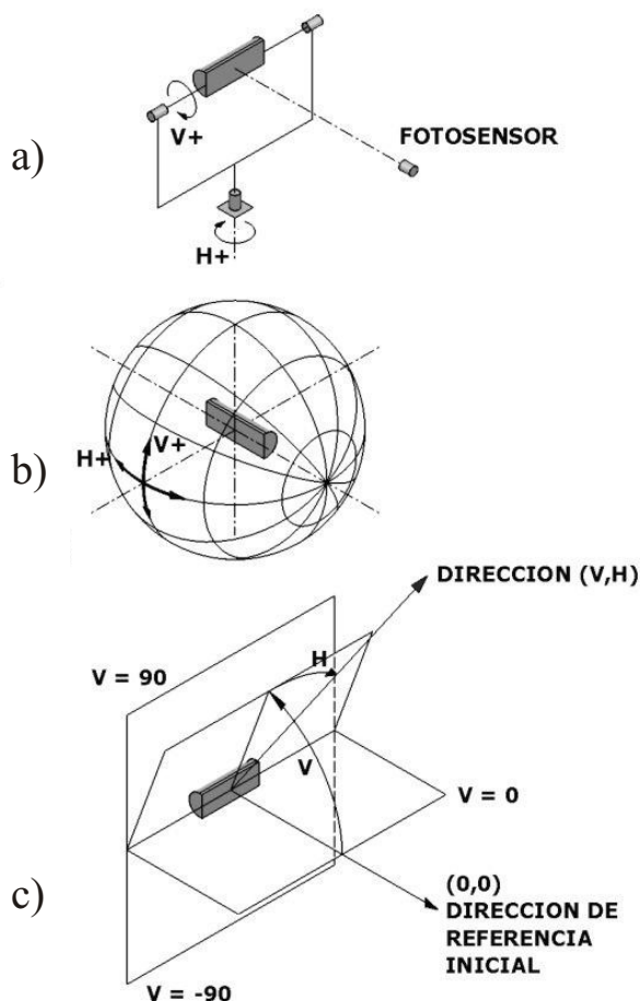
Figura 3. Fotogoniómetro tipo C. (Adaptado de IES Lighting Handbook, 1987, Illuminating Engineering Society of North America).
