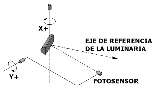
Figura 3. Fotogoniómetro tipo C. (Adaptado de IES Lighting Handbook, 1987, Illuminating Engineering Society of North America).
