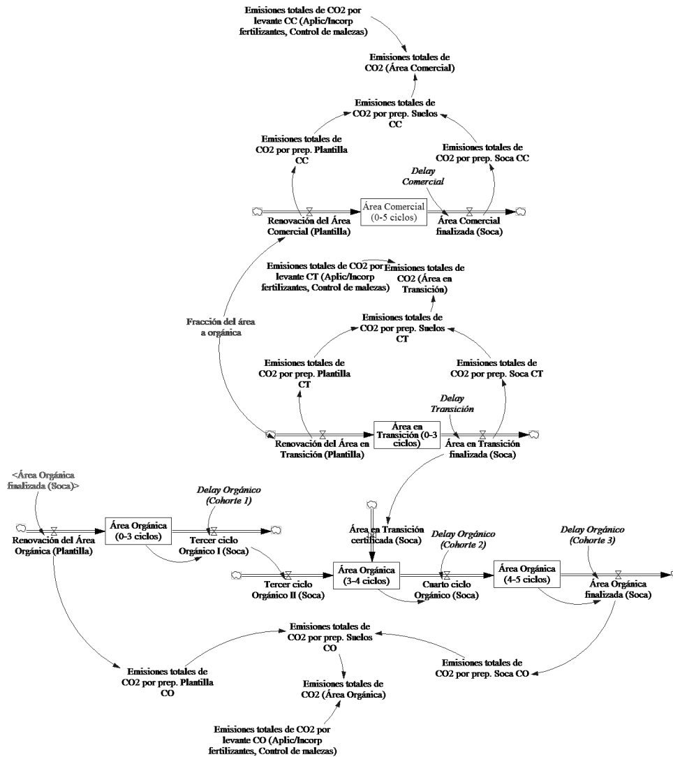
Annex I. Dynamic model of CO2 emissions by fossil fuel combustions. Summarized version.
