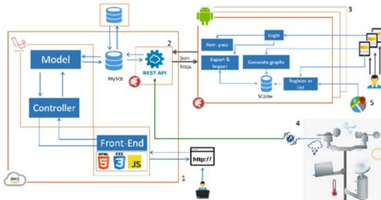
Figure 4. SARA Architecture
