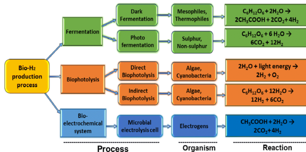
Figure 3. General map of the biological production processes of bio-H 2 . Source: (26).
