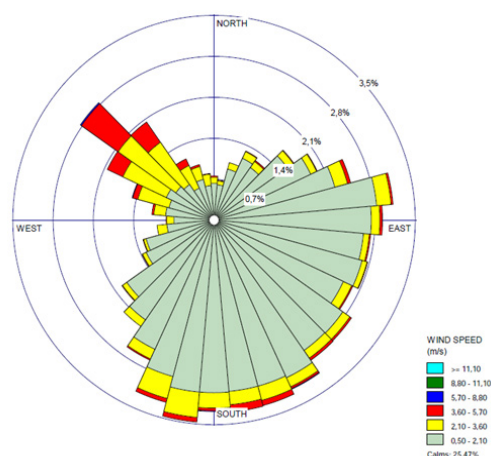
Figure 2. Wind rose
