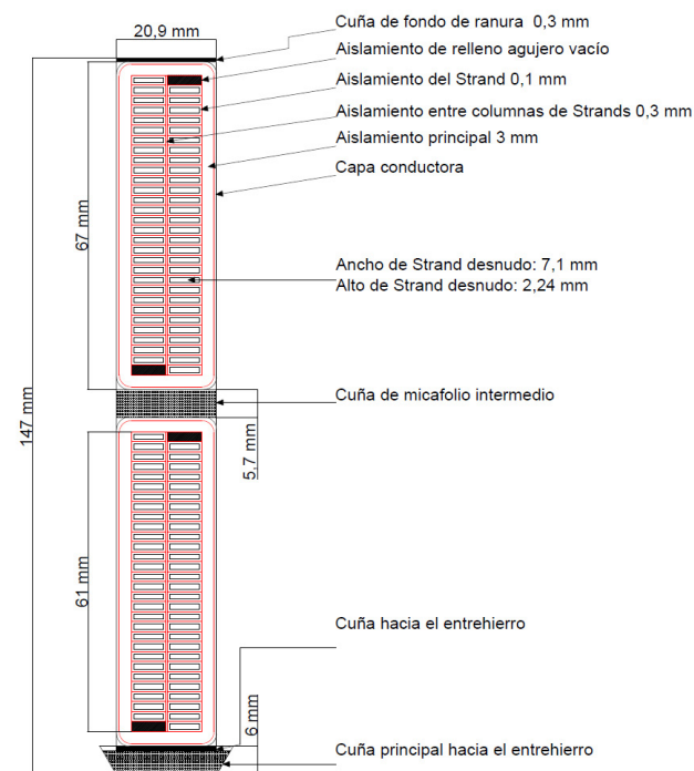
Figure 7. Dimensions of the Abramov method. Source: [5]
