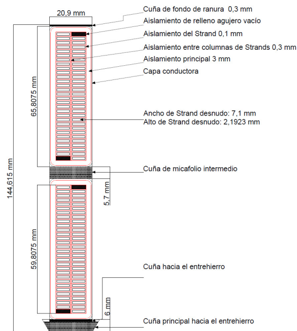
Figure 5. Dimensions of the Juan Corrales method. Source: [5]
