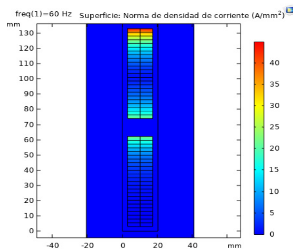
Figure 3. Transversal section of a strained bar without transposition simulated in COMSOL MULTIPHYSICS. Source: [5]
