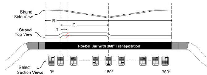
Figure 4. Position of the transposed strand along the Roebel transposition at 180° and 360°. Source: [3].
