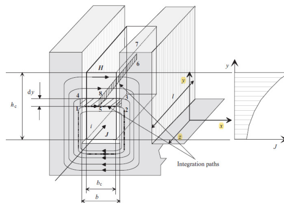
Figure 1. Effect of current displacement in a conductor. Source: [4].
