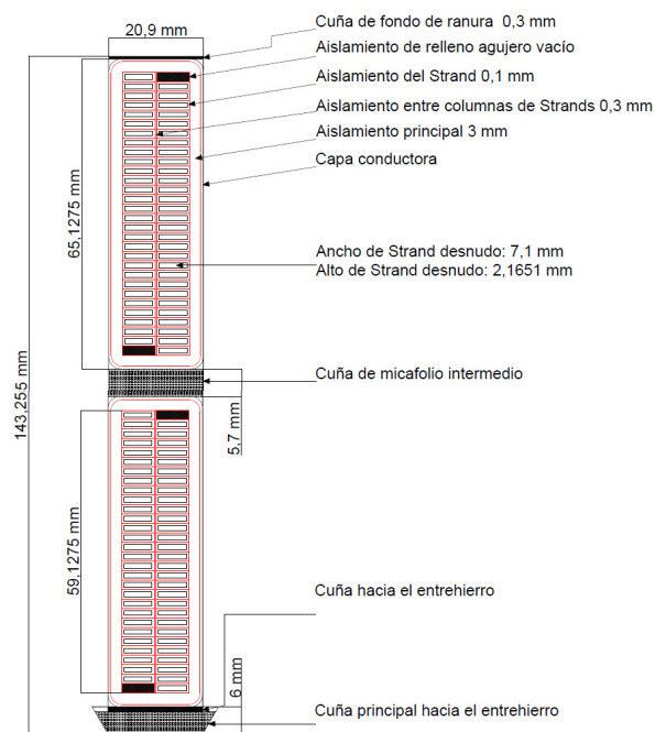
Figure 6. Dimensions of the Karl Vogt method. Source: [5]
