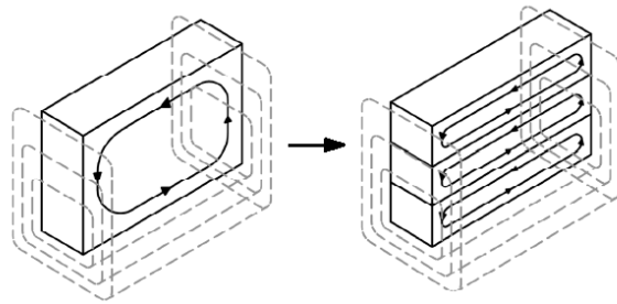
Figure 2. Potential difference compared between an unstrained conductor Vs a strained conductor. Source: [3].
