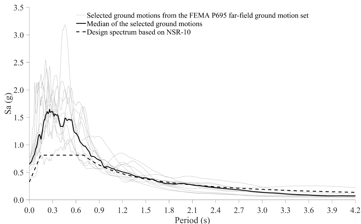
Figure 4 Design spectrum and spectra of the selected records from the FEMA P695 far-field set [28].
