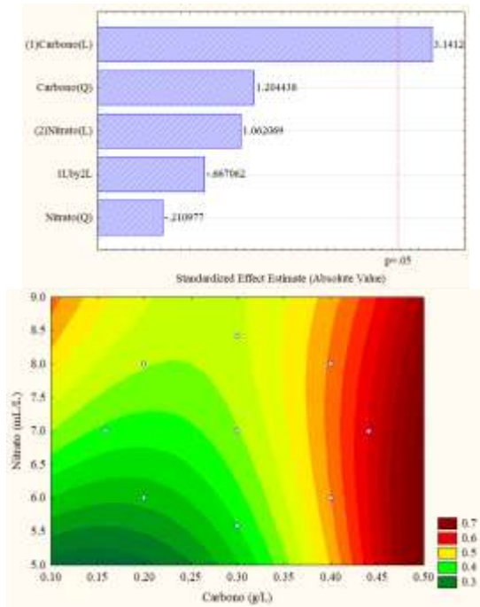
Figure 4b. Pareto diagram and surface response graphic for sodium carbonate/sodium nitrate
